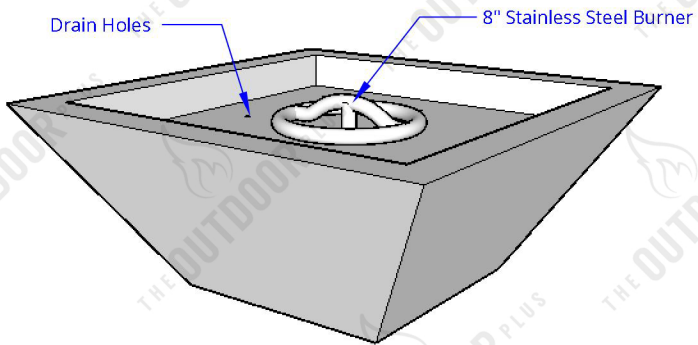
ISOMETRIC VIEW
